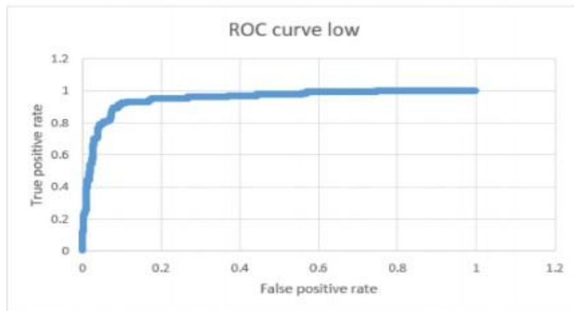
Figure 4 Receiver characteristic curve (class low)
