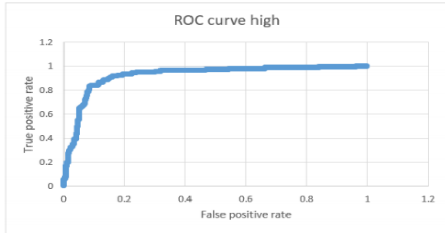
Figure 2 Receiver Characteristic curves (class high)
